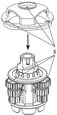
SRAM S7 mounting aid Part No. 65 0324 103 000
